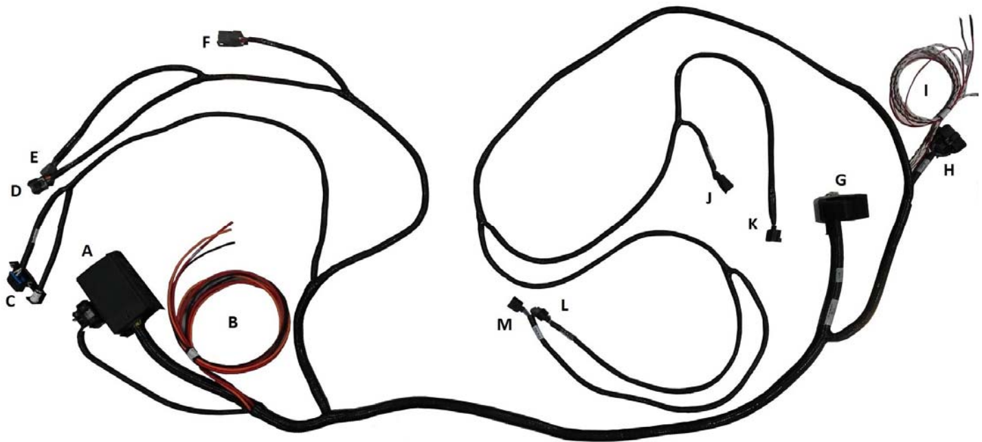
Figure 1 - Controls Pack Wiring Harness Components
