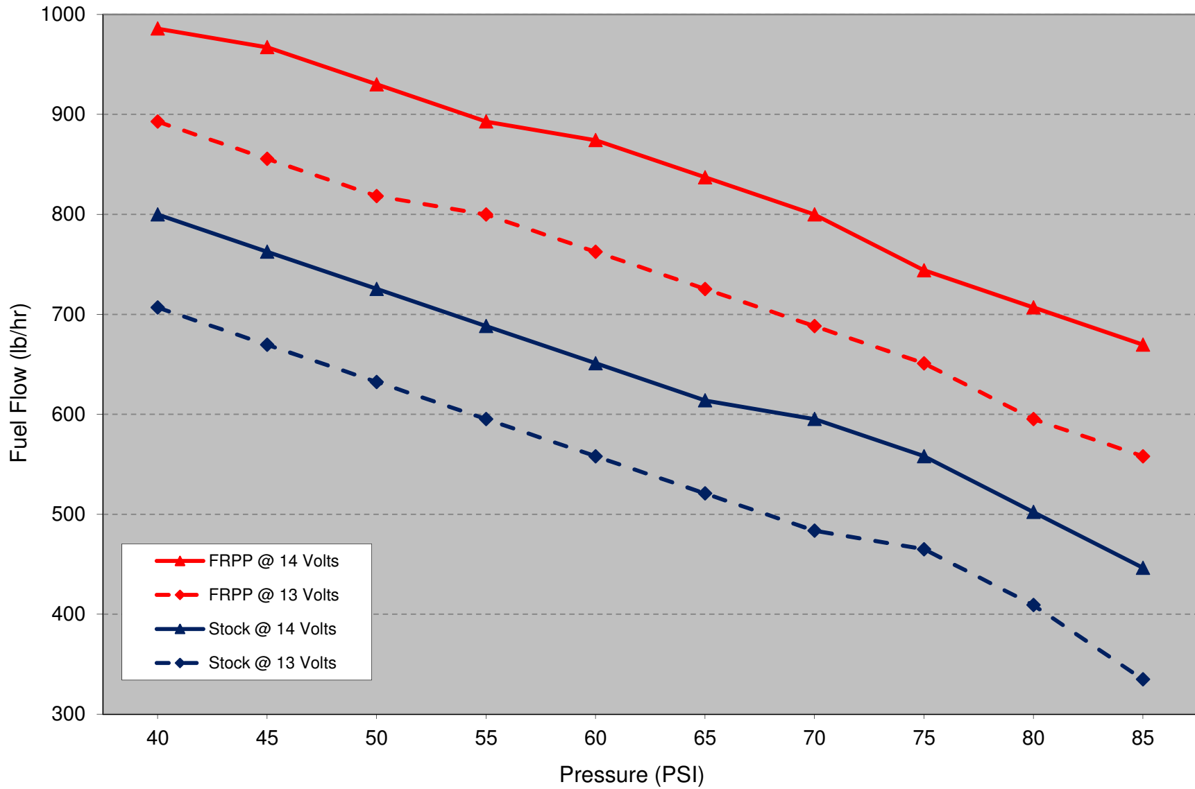
M-9407-MSVT Fuel Flow vs Stock 2013-2014 GT500
